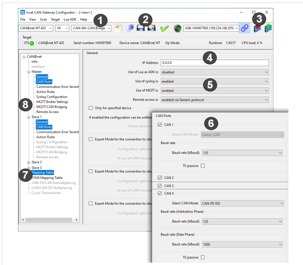
Fig. 9 CAN-Gateway Configurator CAN@net NT 420
